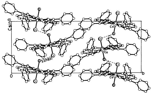
Fig. 2. The crystal structure projected along the a axis. Hydrogen atoms are omitted for clarity. Broken lines show the O-H...Cl hydrogen bonds (distances in Å).
